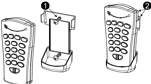
Figure 2 - Mounting
