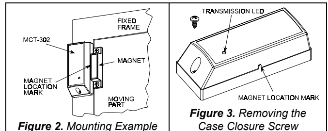
Figure 2. Mounting Example
